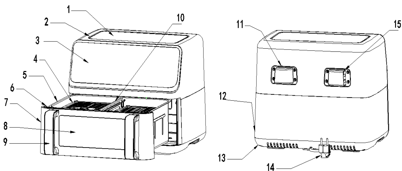
FIG. 1 : Details of Air Fryer
