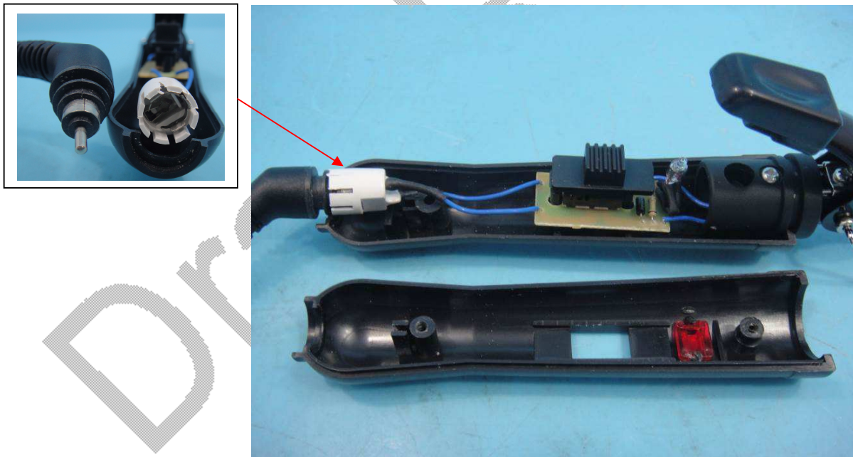
Photo 4: inside view
