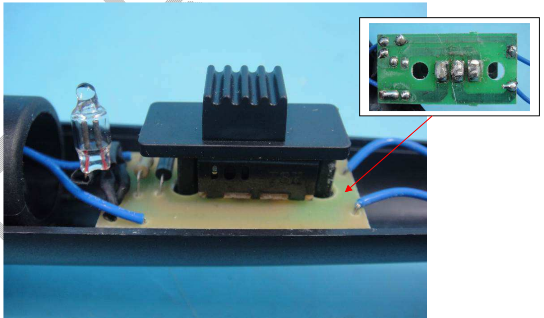
Photo 6: PCB view
