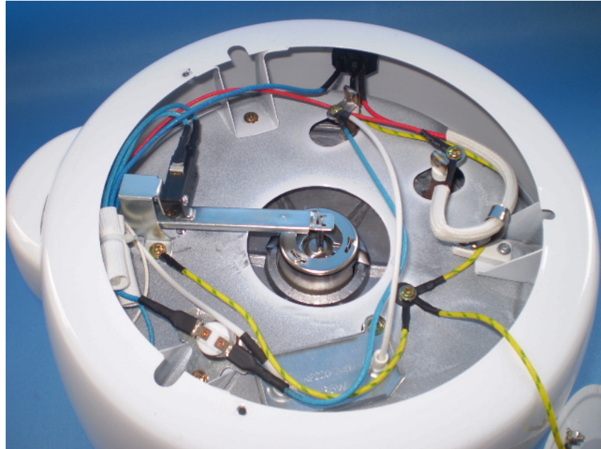
Fig. 11: Inner view, appliance inlet used and temperature limiter Y with micro switch
