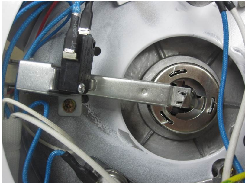
Fig. 14: Temperature limiter for all models with suffix M
