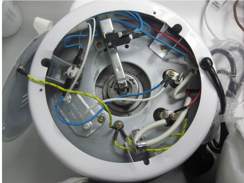
Fig. 9: Inner view, Type Y cord connection and temperature limiter Y with micro switch
