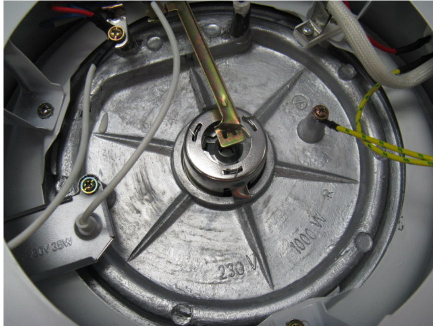
Fig. 21: Heating element
