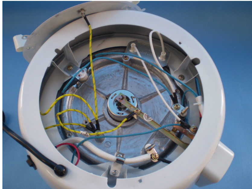
Fig. 10: Inner view, Type Y cord connection and temperature limiter R without micro switch
