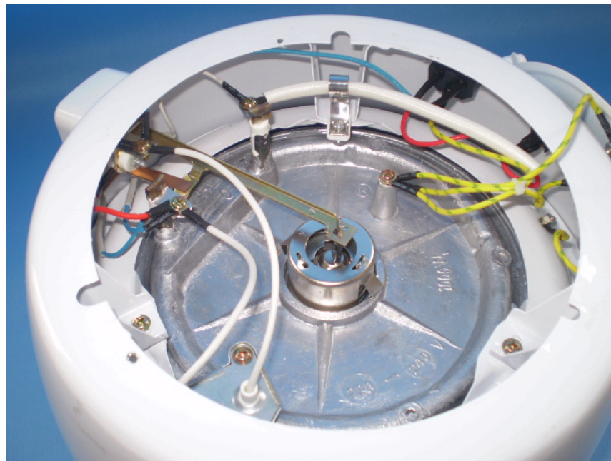
Fig. 12: Inner view, appliance inlet used and temperature limiter without micro switch
