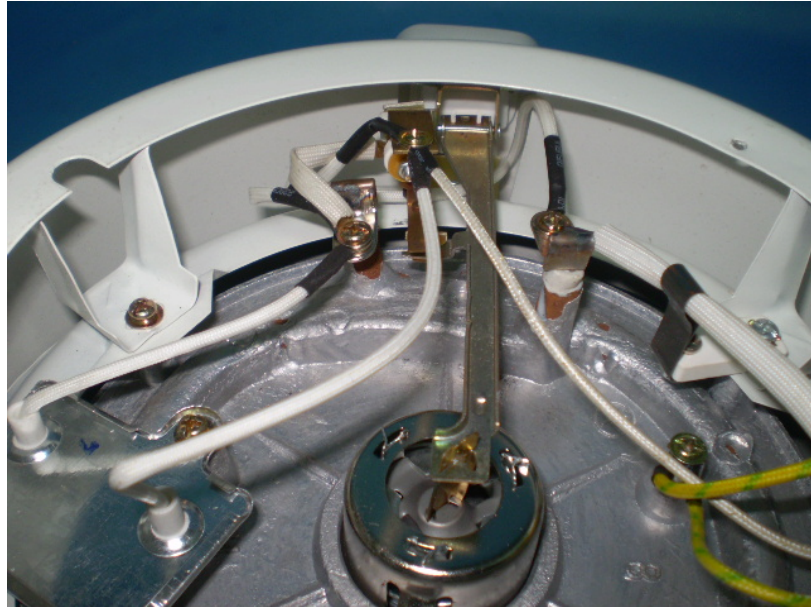
Fig. 13: Temperature limiter for all models without suffix M
