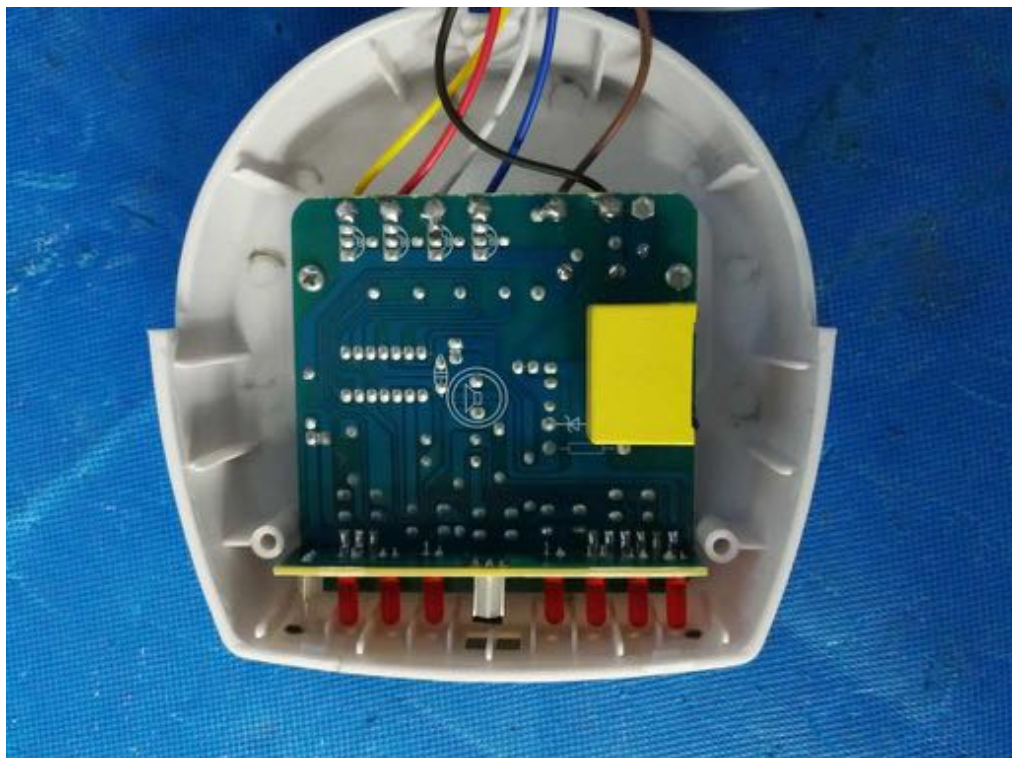
Control PCB
